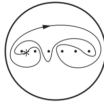
FIGURE 3. The curve \mathcal{C} of Example 4.
